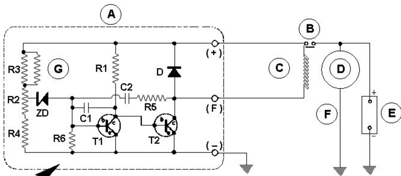
4TR Control Unit Circuit Diagram
